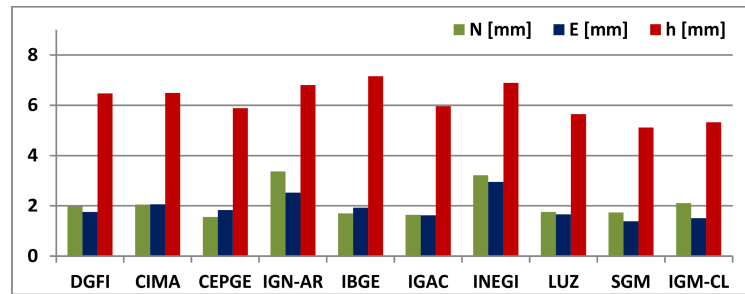
Figure 4: Mean RMS values for the weekly repeatability of station positions in the solutions delivered by the SIRGAS Analysis Centres (Time span: GPS weeks 1641–1705).
