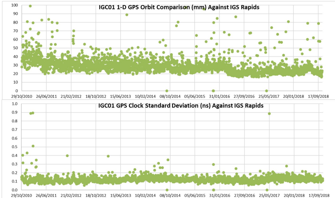
Figure 8: IGC01 ESOC combined solution performance of GPS orbit and clock solutions. Top: 1 day orbit comparison against IGS rapid products [mm]. Bottom: GPS clock standard deviation against IGS rapid products [ns].
